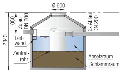
Sedimentationsanlage ViaSed
