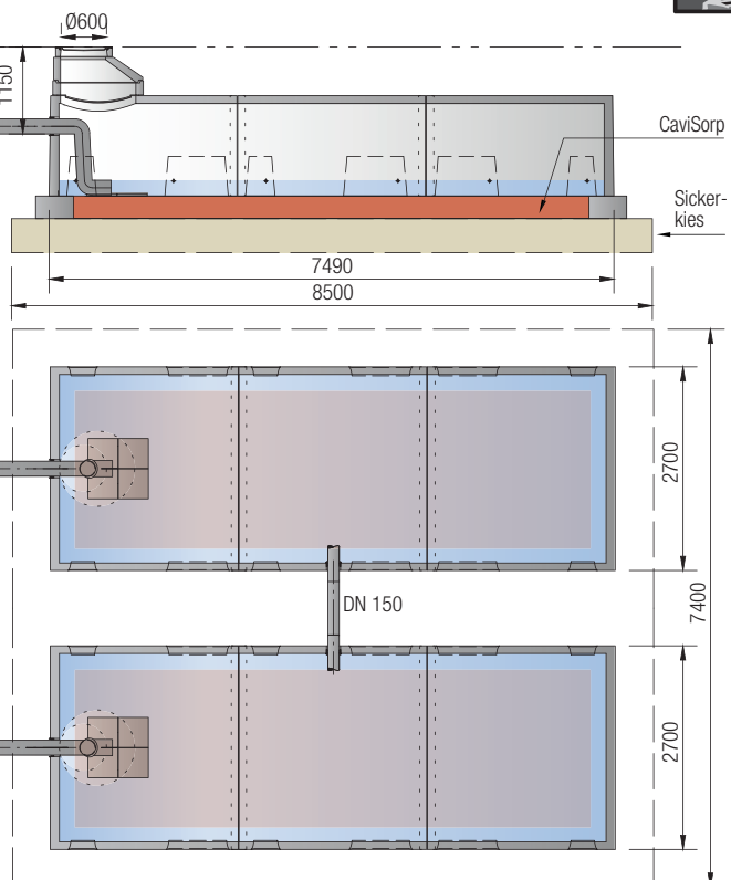
Sickertunnel CaviLine Sorp
