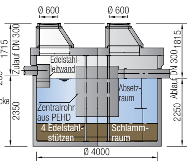
Sedimentationsanlage ViaSed
