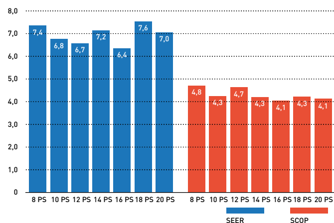
SEER / SCOP
