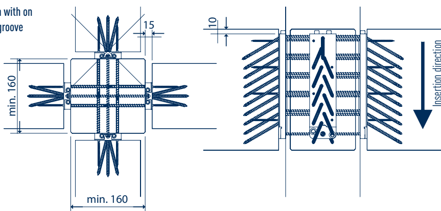
4-fold on support connection milled
