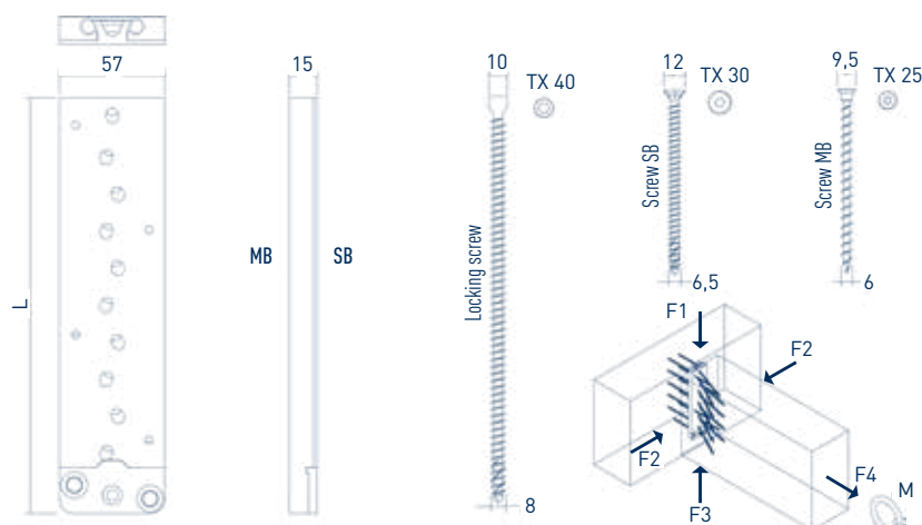
SIHGA® Dimension Main beam Secondary beam
