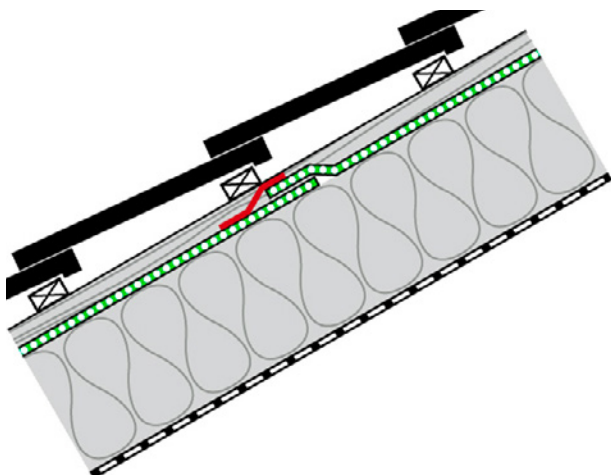
Überlappung
